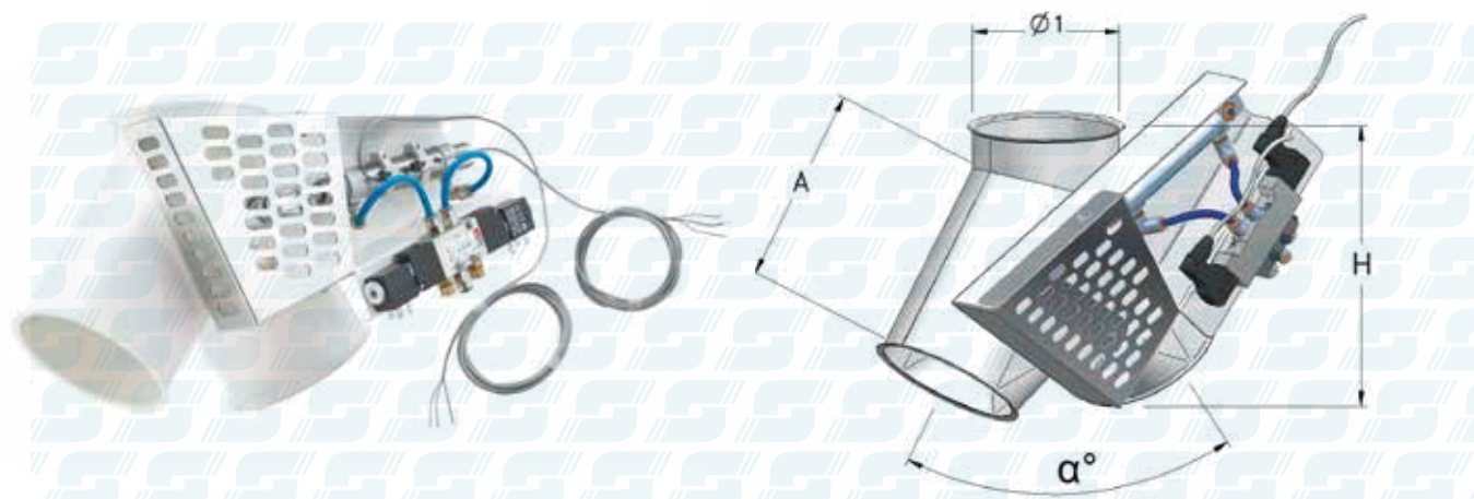
Valvole Simmetriche a due vie 30°+30° / Comando EPN - Diverter valves symmetric 30°+30° electro-pneumatic operated
